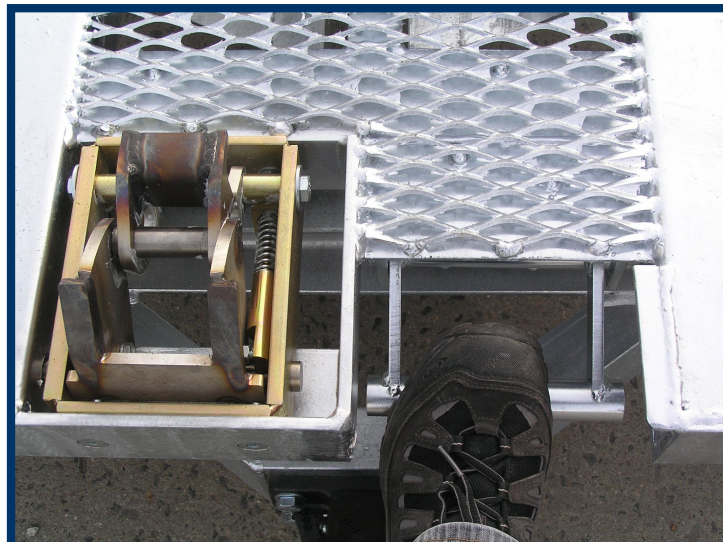
... foldable by pedals located on opposite side of platform.
